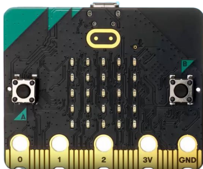
Microbit
